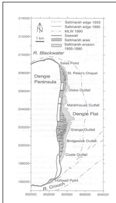
Figure C.2 Changes in the position of the saltmarsh edge along the Dengie Peninsula, Essex, between 1955 and 1990, based on Ordnance Survey maps and aerial photographs (after Pye and French, 1993)
